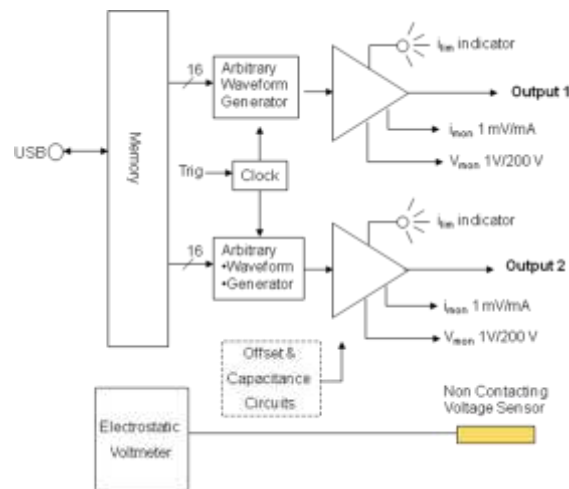
Figure 10. Typical block diagram of the Trek electrostatic Chucking Amplifier products
