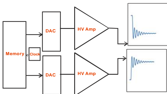
Figure 3. The arbitrary waveform generator and the high voltage amplifier working together
