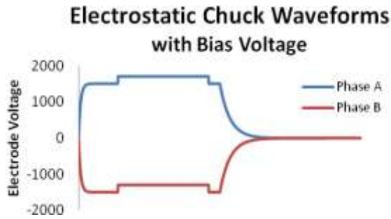
Figure 6. Application of a bias voltage.
